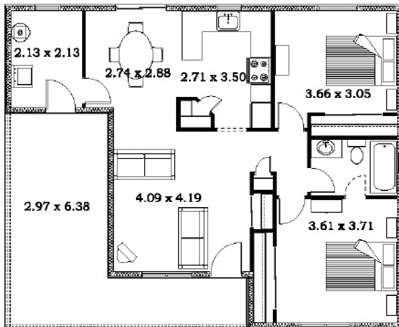
Floor Plan
